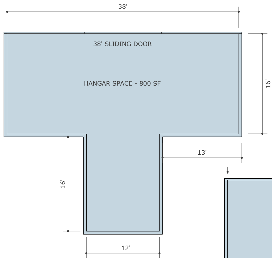
100 - 400 BUILDINGS (32)
