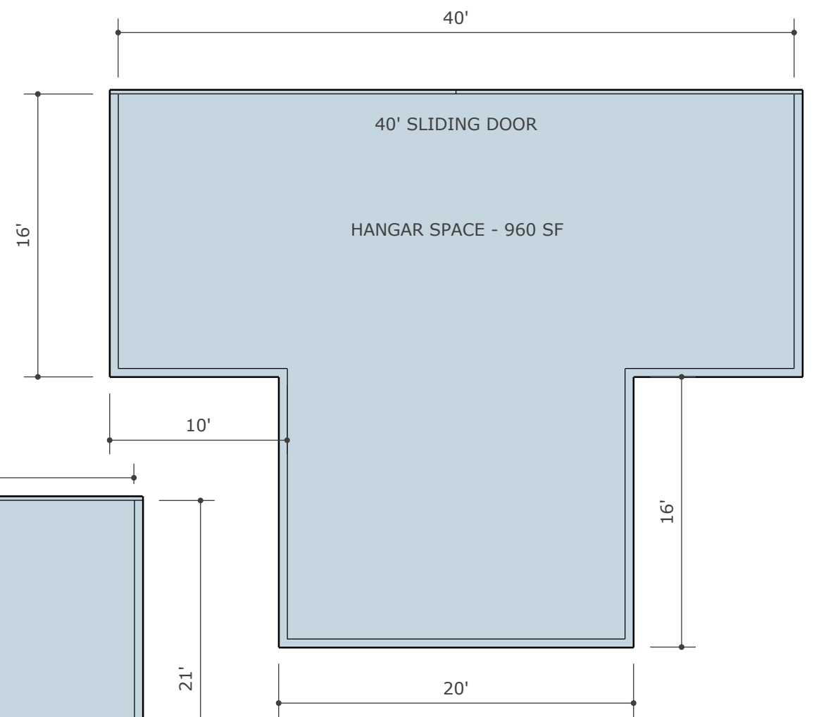
700 BUILDING - SINGLES (13)
